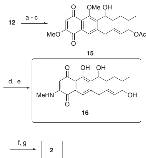
Scheme 3. Reagents and conditions: (a) \text{Ac}_2\text{O} , Pyr., \text{CH}_2\text{Cl}_2 , rt; (b) DDQ, t -BuOH, aq. \text{CH}_2\text{Cl}_2 , 0 °C; (c) \text{BBR}_3 , \text{CH}_2\text{Cl}_2 , -78 °C, 16% from 12 ; (d) \text{MeNH}_2 , THF, 0 °C; (e) \text{K}_2\text{CO}_3 , MeOH, rt, 87% in 2 steps; (f) \text{MnO}_2 , \text{CH}_2\text{Cl}_2 , 40 °C; (g) PDC, DMF, rt, 19% from 16 ; Jones reagent, acetone, -20 °C, 43% from 16 .
